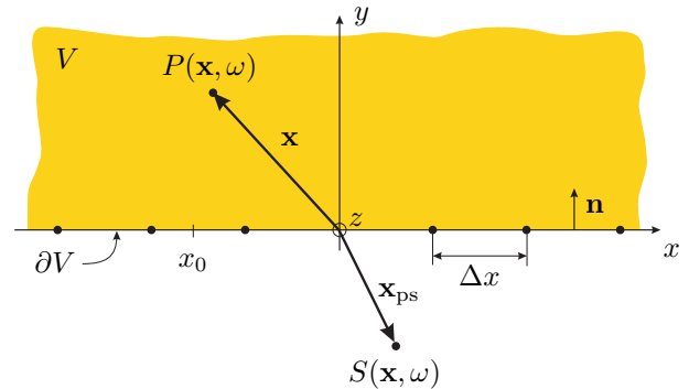
Fig. 1: Geometry underlying the derivation of WFS and the SDM. The reproduction of a virtual point source placed at \mathbf{x}_{ps} using a linear distribution \partial V of secondary point sources located on the x -axis is considered. The yellow area V denotes the listening area, the z -axis points out of the illustration plane.
