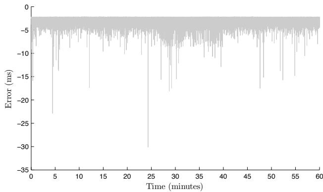
Figure 1. Error in the observed global clock for a single slave.
